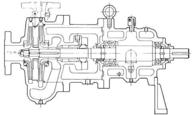
SDH MODEL
